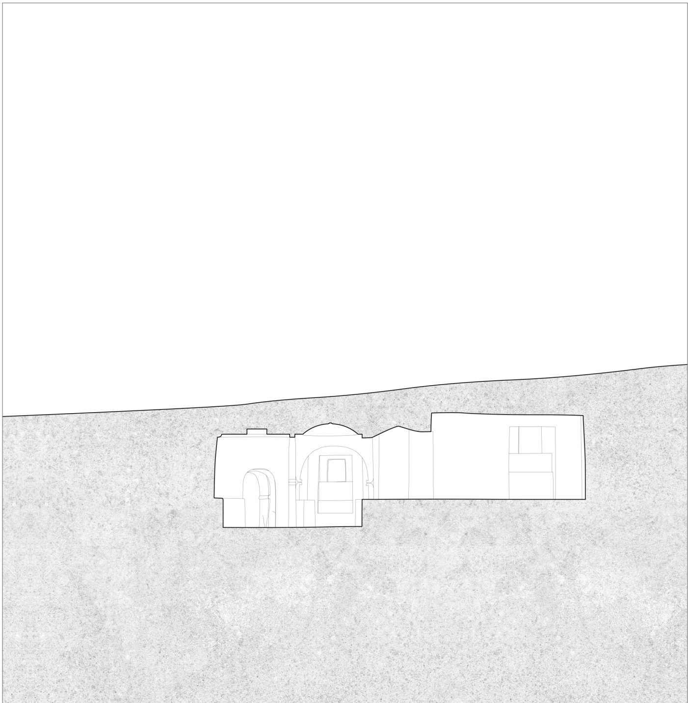
Dagmawi Lalibela (Ambager Complex) Section XX (2017)
